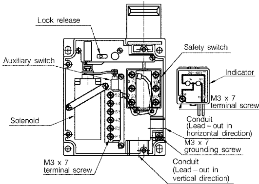
LJS-E5312
