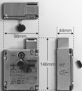
For details on dimensions, see relevant drawings.
